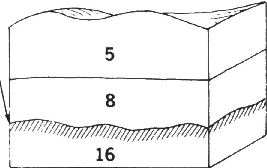
Outcrop 6
