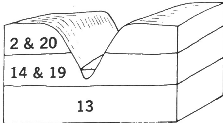
Outcrop 4
