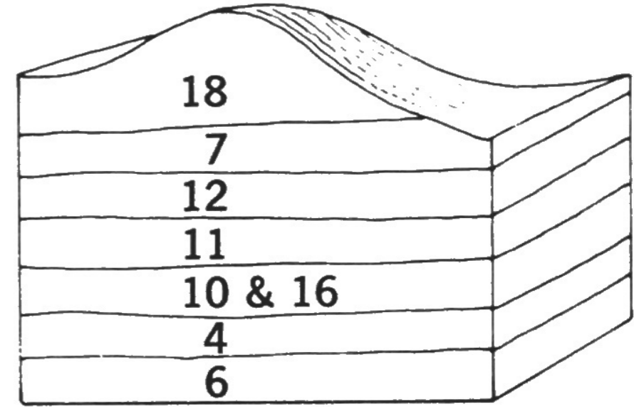
Outcrop 3
