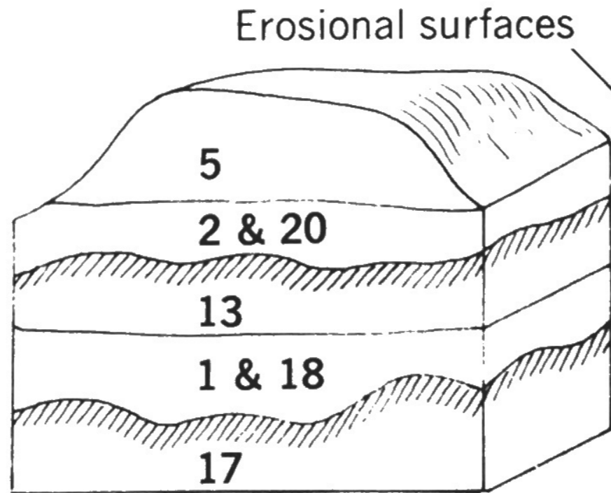
Outcrop 5
