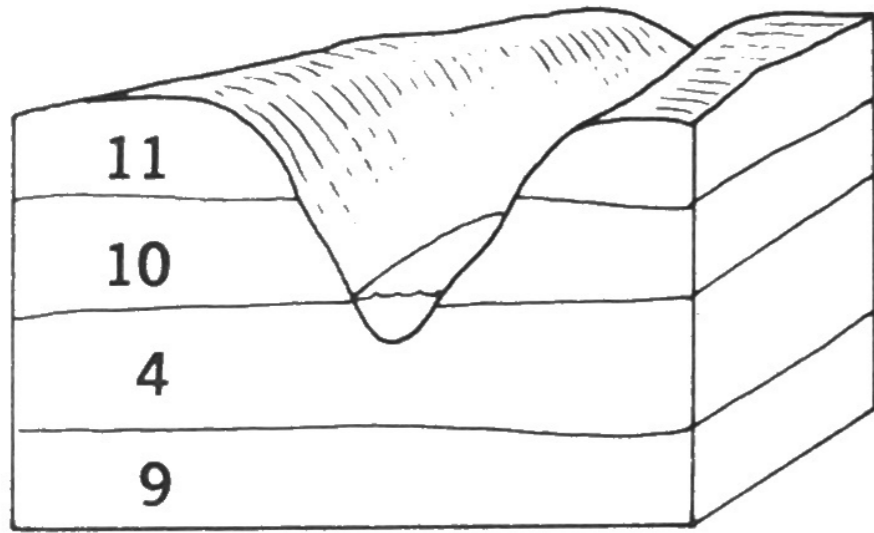
Outcrop 1
