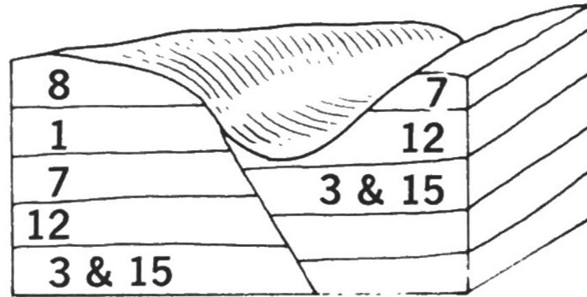
Outcrop 2
